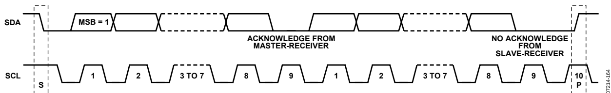
Figure 59. Data Transfer Process (Master Read Mode, 2-Byte Transfer Used for Illustration)
