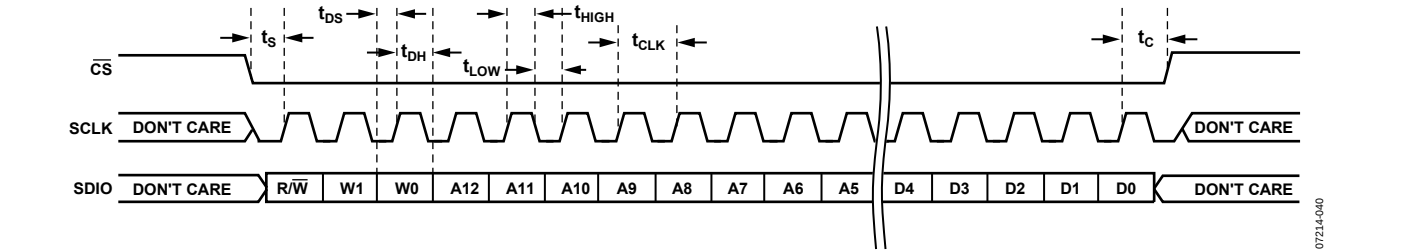
Figure 65. Serial Control Port Write—MSB First, 16-Bit Instruction, Timing Measurements
