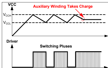
Figure 2: VCC Start-Up
