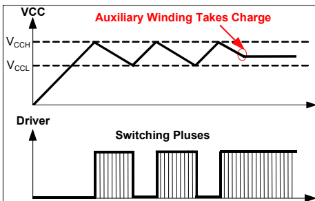
Figure 2: VCC Start-Up
