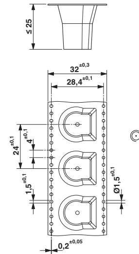
Dimensional drawing
