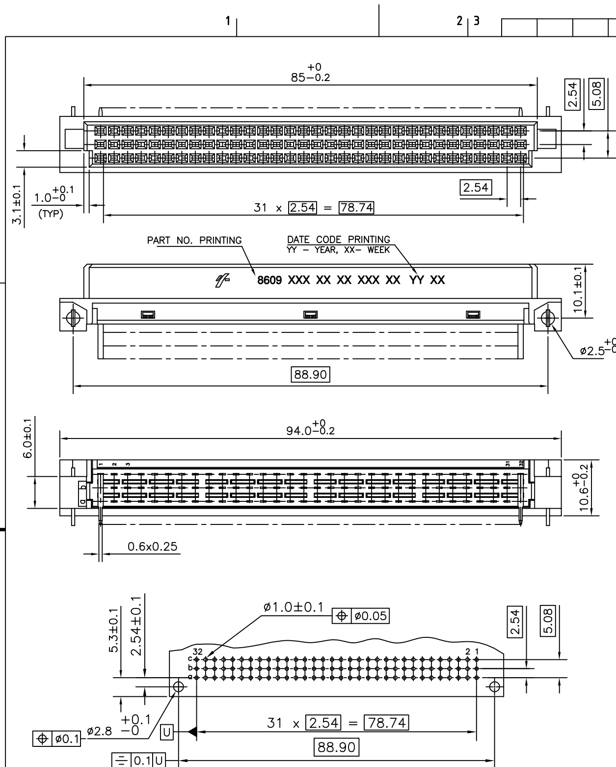
PCB DRILLING DETAILS
