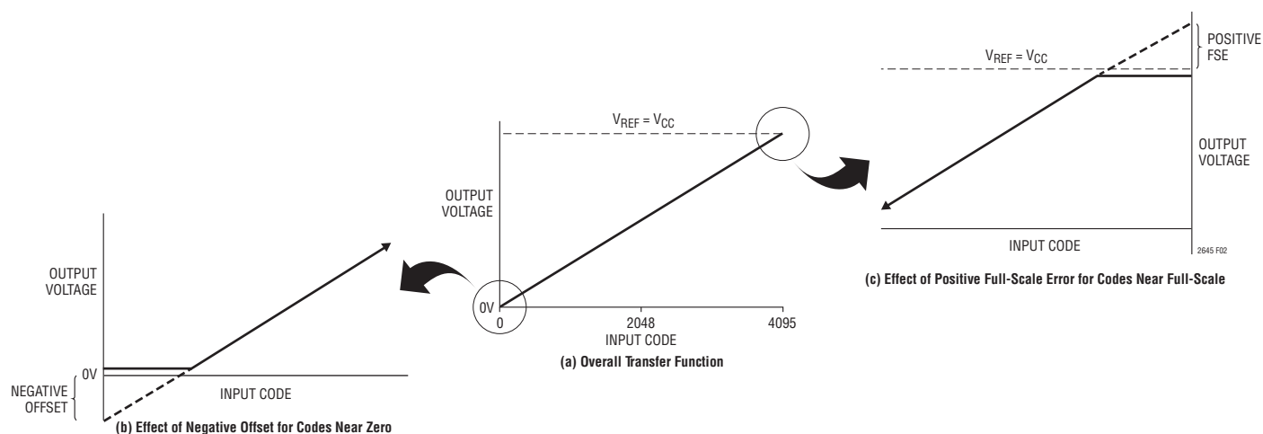
Figure 2. Effects of Rail-to-Rail Operation on a DAC Transfer Curve (Shown for 12 Bits)
