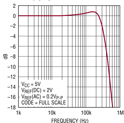
Multiplying Bandwidth
