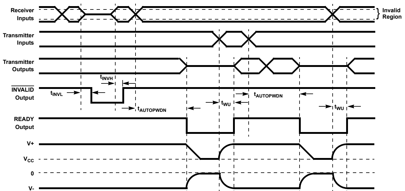
Figure 13. Enhanced Automatic Powerdown, \overline{\text{INVALID}} , and READY Timing Diagrams
