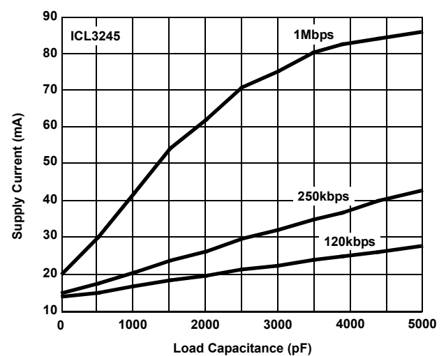
Figure 4. Supply Current vs Load Capacitance When Transmitting Data
