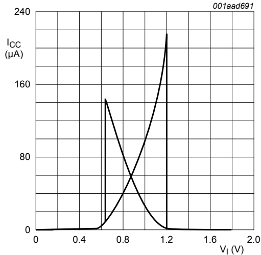
Fig. 10. Typical transfer characteristics; V_{CC} = 1.8 \text{ V}
