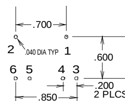
MOUNTING HOLE PATTERN TOP VIEW
