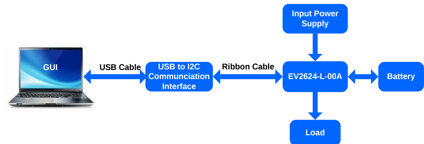
Figure 1: EVKT-2624 Evaluation Kit Set-Up
