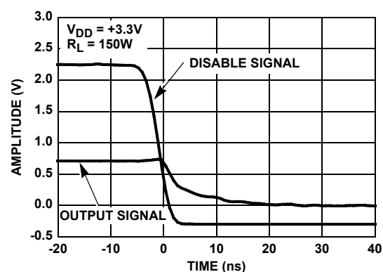
FIGURE 14. DISABLE TIME
