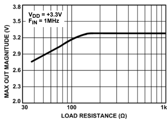
FIGURE 9. MAXIMUM OUTPUT vs LOAD RESISTANCE
