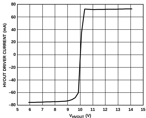
Figure 29. HVOUT VHH Current Limit; V_{HH} = 10.0 V; V_{HVOUT} Swept from -5.9 V to +14.1 V
