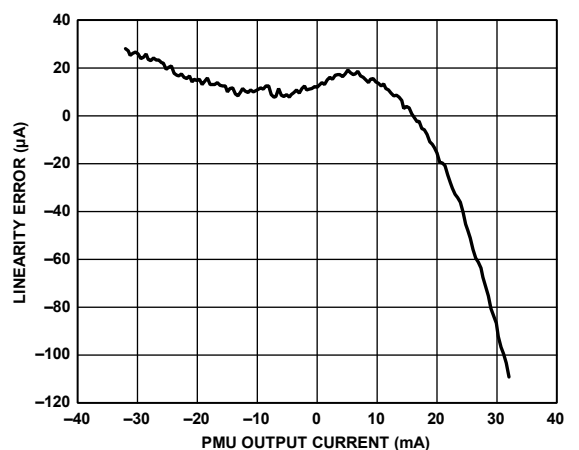
Figure 43. PMU Force Current Range A Linearity
