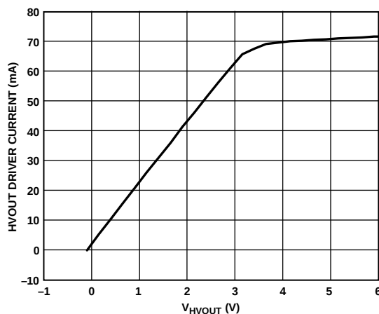
Figure 28. HVOUT VH Current Limit; V_H = -0.1 V; V_{HVOUT} Swept from -0.1 V to +6.0 V
