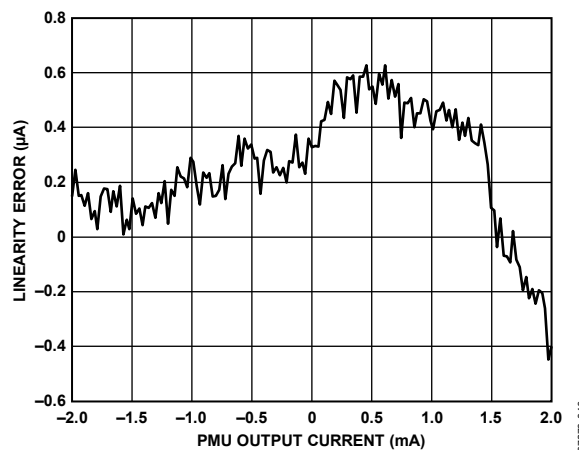
Figure 44. PMU Force Current Range B Linearity
