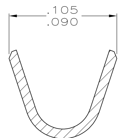
SECTION X-X INSULATION BARREL SCALE 20:1
