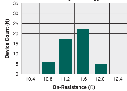
Typical On-Resistance Distribution (N=50, I_L=170mA_{DC} )
