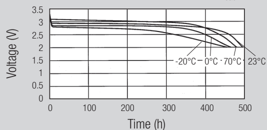
Temperature performance Load 47 kΩ
