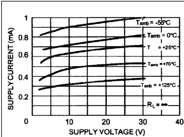
Figure 2. Supply current versus supply voltage
