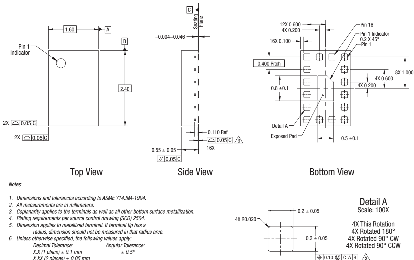
Figure 11. SKY13551-668LF Package Dimensions
