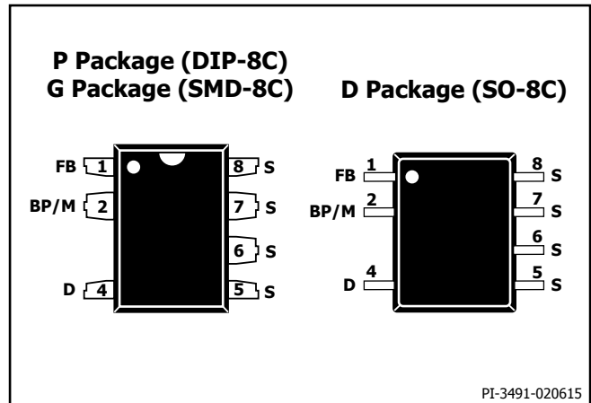
Figure 4. Pin Configuration.
