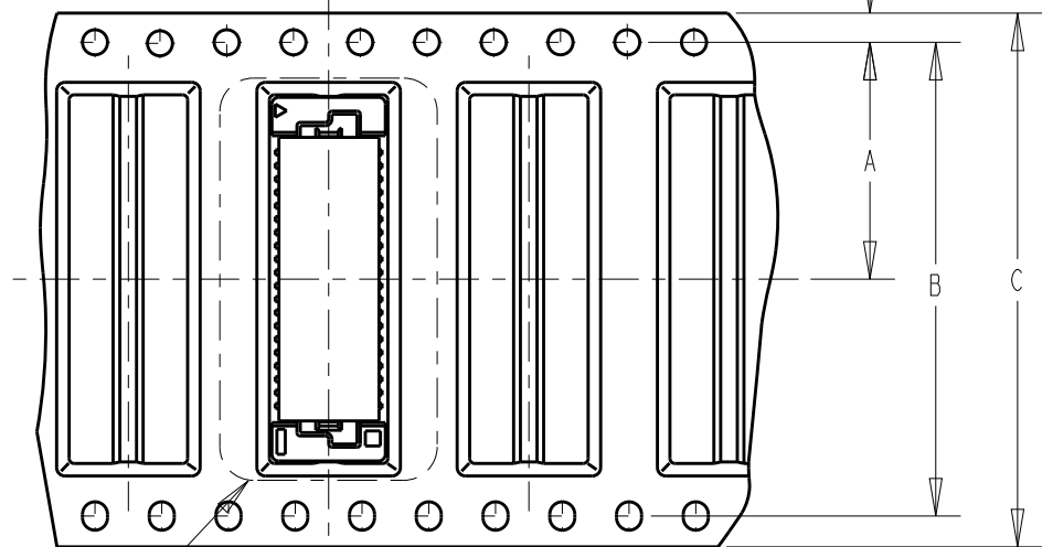
DETAIL B
