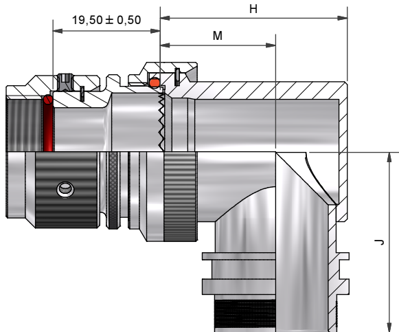
90° BACKSHELL - TYPE 2
