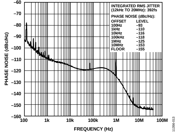
Figure 14. Absolute Phase Noise (Output Driver = LVPECL), f_R = 49.152 MHz Crystal, f_{OUT} = 693.482991 MHz on Both PLLs
