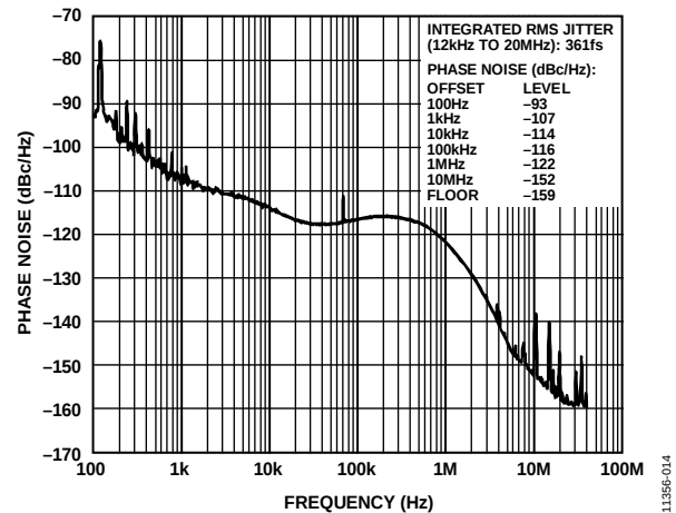
Figure 15. Absolute Phase Noise (Output Driver = LVPECL), f_R = 49.152 MHz Crystal, f_{OUT} = 919 MHz on Both PLLs
