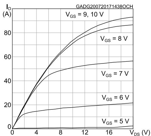
Figure 6: Output characteristics
