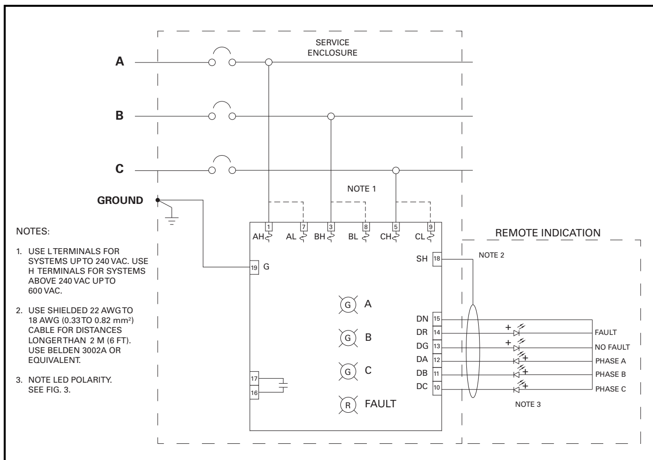
FIGURE 2. Connection Diagram.
