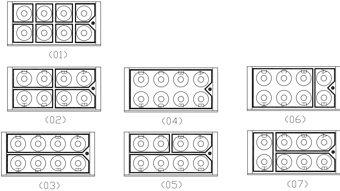
BUSSING ARRANGEMENTS 3
