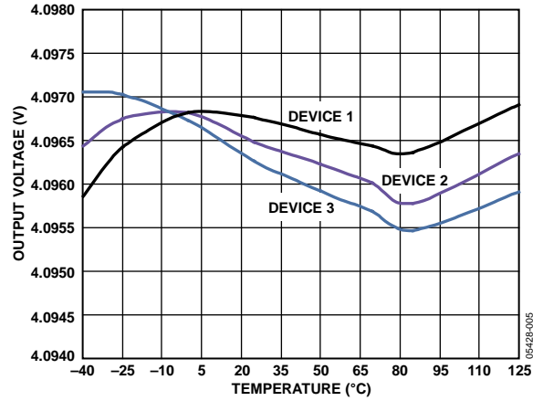
Figure 8. ADR444 Output Voltage vs. Temperature
