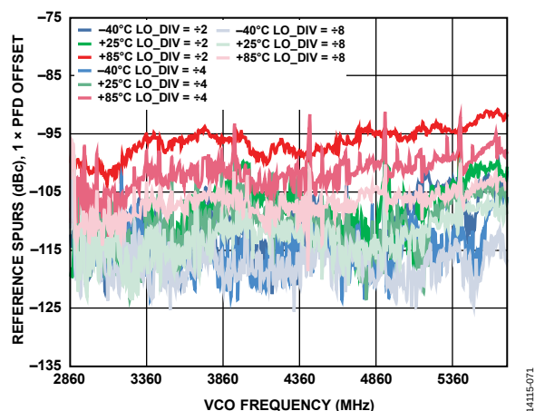
Figure 87. f_{PFD} Reference Spurs vs. VCO Frequency, 1 \times PFD Offset, Measured at LO Output, Integer Mode
