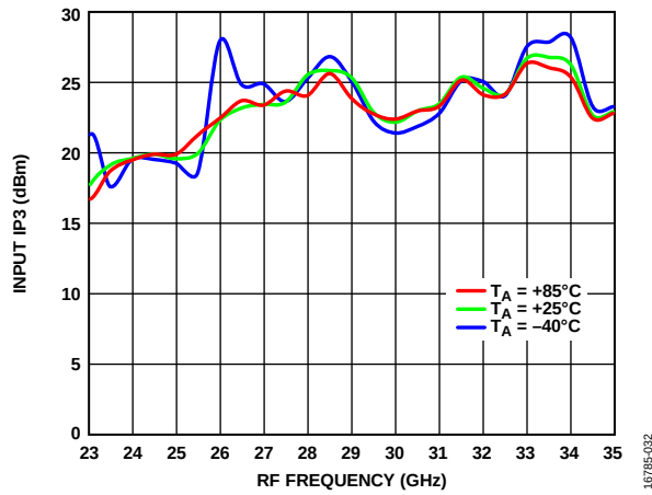
Figure 32. Input IP3 vs. RF Frequency at Various Temperatures, LO = 4 dBm
