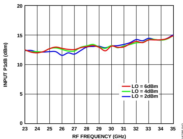
Figure 46. Input P1dB vs. RF Frequency at Various LO Power Levels, TA = 25°C
