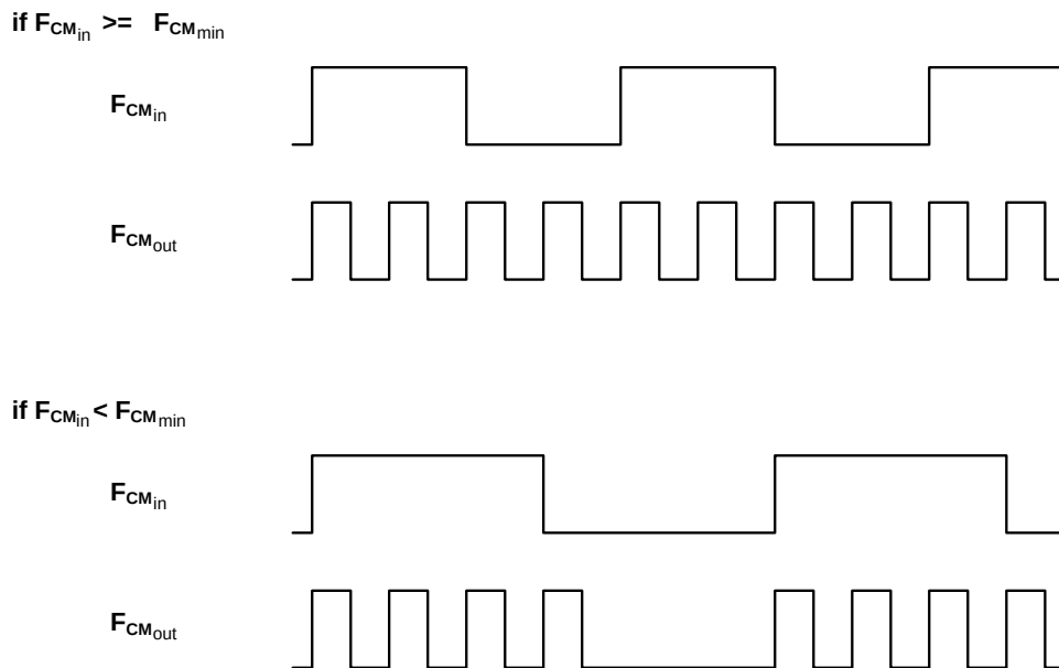
Figure 18.2. Example Clock Multiplier Output
