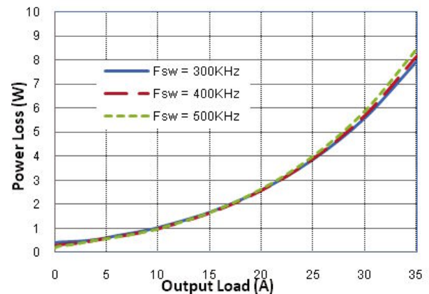
Typical Power Loss V_{IN} = 12\text{ V} , V_{OUT} = 1.2\text{ V} , V_{DRV} = V_{CIN} ; NO AIR FLOW, O/P Inductance = 0.33 \mu\text{H}
