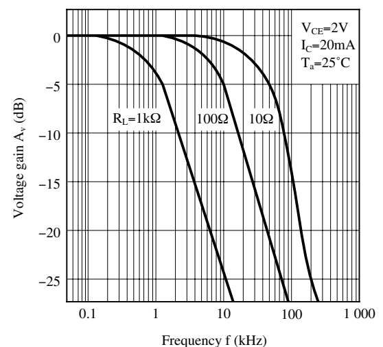
Fig.12 Frequency Response
