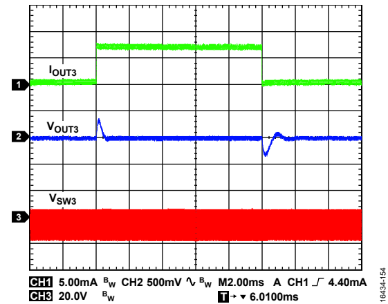
Figure 50. Inverting Regulator Load Transient Response, V_{OUT1} = +6 V , V_{OUT3} = -15 V , I_{OUT2} = -0.3 mA to -7 mA Step, T_A = +25^\circ C
