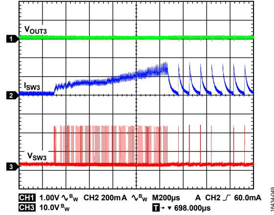
Figure 49. Inverting Regulator Short-Circuit Current Limit During Startup, V_{OUT1} = +24 V , V_{OUT3} = SGND2 , T_A = +25^\circ C
