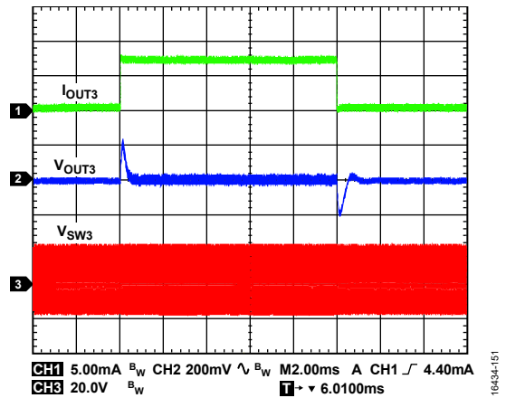
Figure 47. Inverting Regulator Load Transient Response, V_{OUT1} = +24 V , V_{OUT3} = -15 V , I_{OUT2} = -0.3 mA to -7 mA Step, T_A = +25^\circ C
