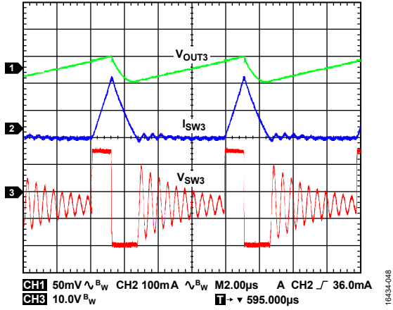
Figure 46. Inverting Regulator Discontinuous Conduction Operation Showing I_{L3} , Switch Node Voltage, and Output Ripple, T_A = +25^\circ C , V_{OUT1} = +24 V , V_{OUT3} = -15 V , I_{OUT3} = -20 mA
