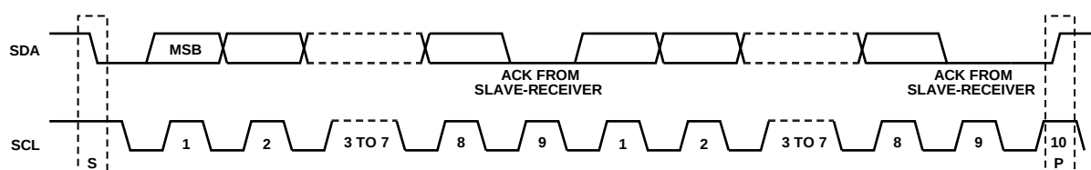
Figure 64. Acknowledge Bit
