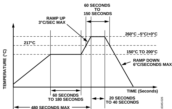
Figure 2. Pb-Free Reflow Solder Profile
