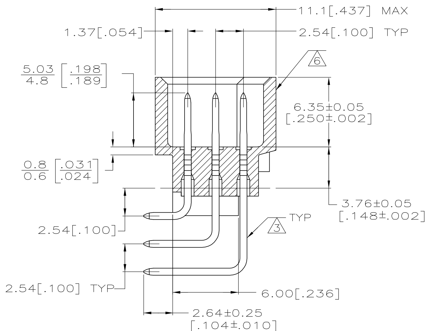
SECTION Z-Z
