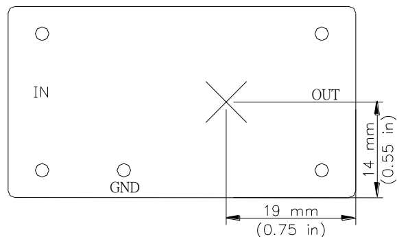
Figure 5: Temperature measurement location The allowed maximum hot spot temperature is defined at 110 °C
