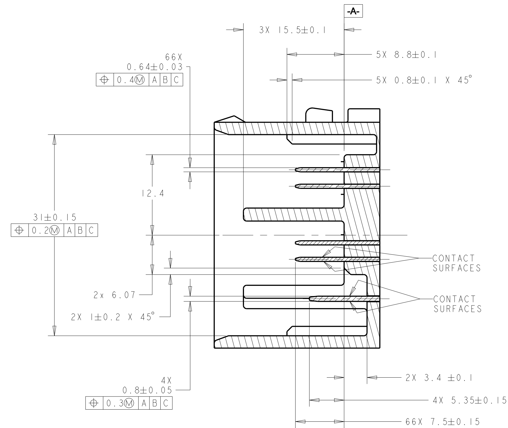
SECTION C-C
