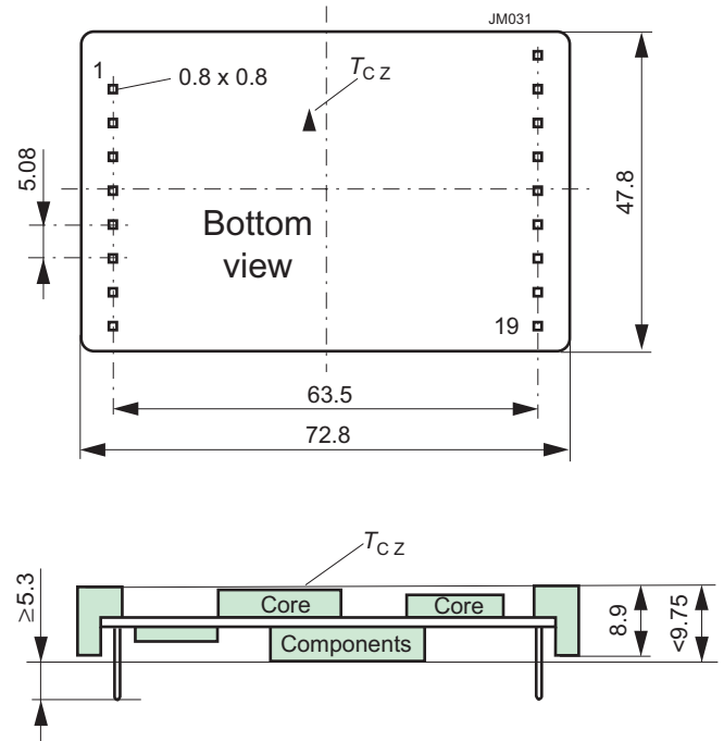
Fig. 14 IMX70/IMY70 open frame (option Z) Weight: approx. 70 g
