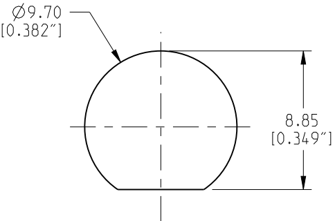
PANEL CUTOUT
