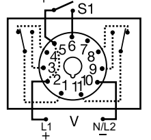
11-pin DPDT
