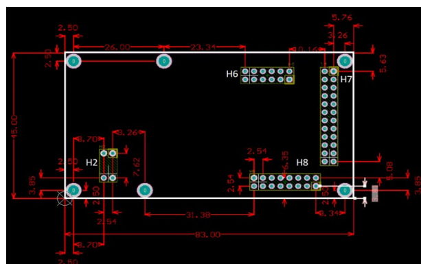
Figure 3: SM2400-EV1Mx-x Top View
