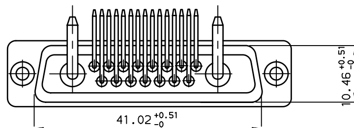
LAYOUT DIMENSIONS (after plating) CONNECTOR SIDE VIEW
