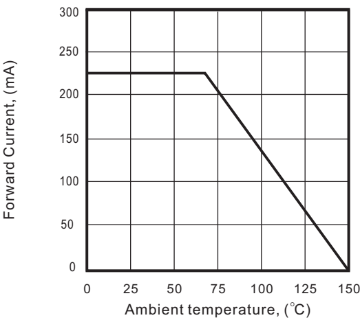
Fig.1- Power derating
