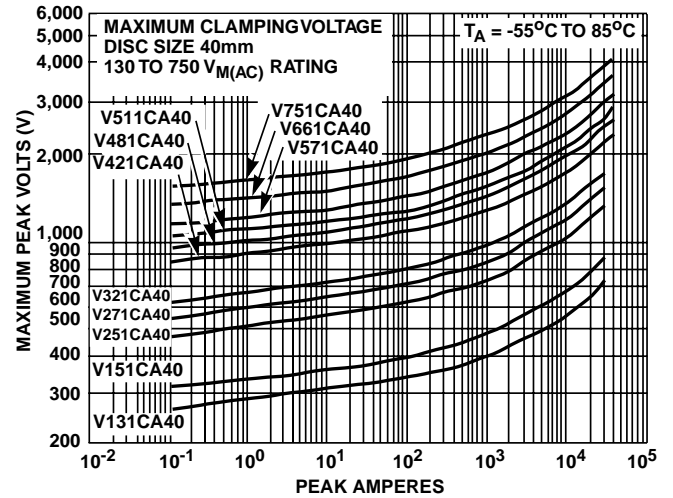
FIGURE 4. CLAMPING VOLTAGE FOR V131CA40 - V751CA40
