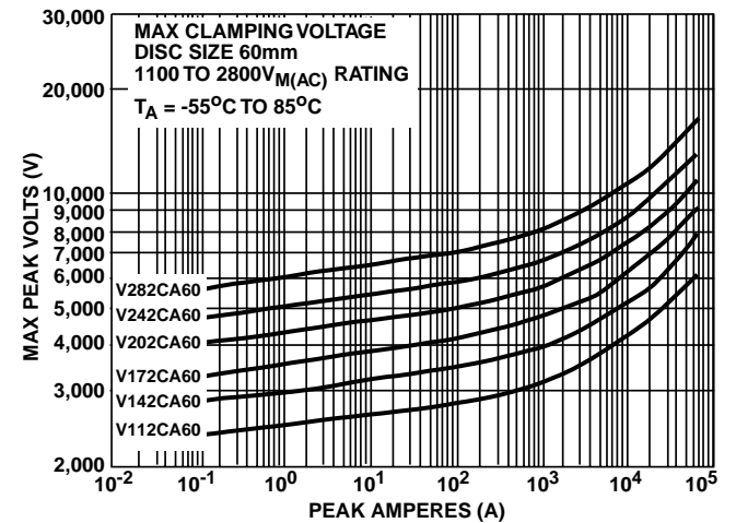
FIGURE 6. CLAMPING VOLTAGE FOR V112CA60 - V282CA60
