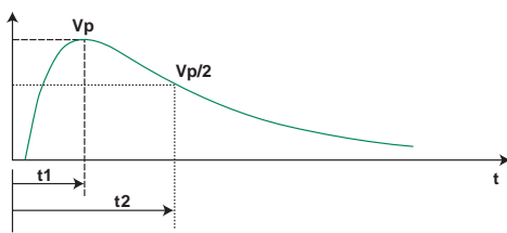
Figure 1. Lightning Transient Waveform
