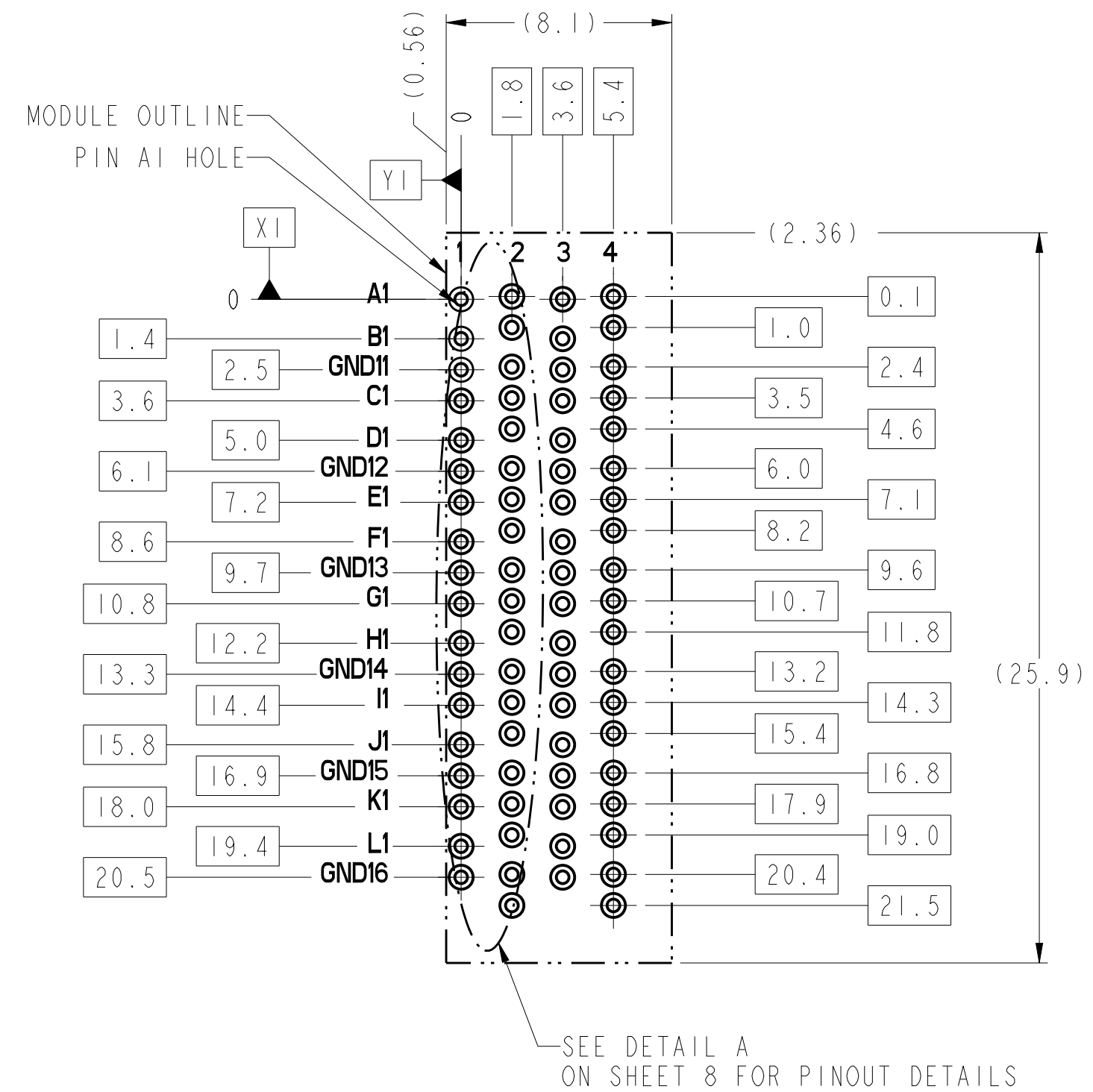
BP HOLE PATTERN COMPONENT SIDE RIGHT WALL MODULE BACKPLANE FOOTPRINT
