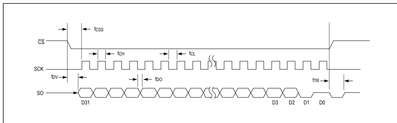
Figure 2. Serial-Interface Timing
