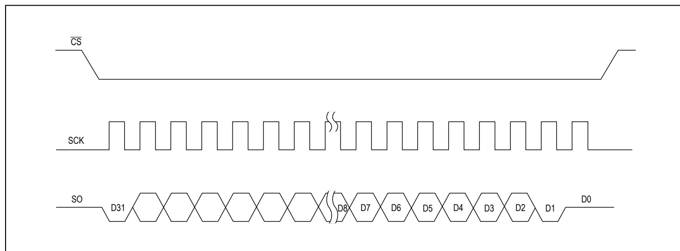
Figure 1. Serial-Interface Protocol
