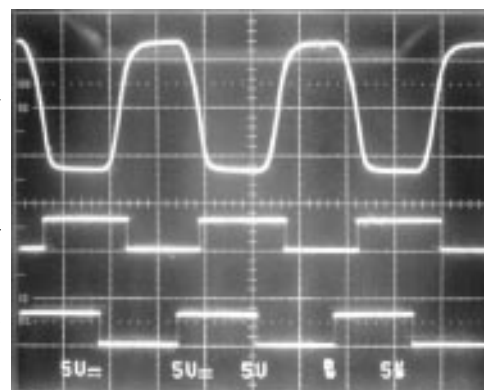
Figure 6. Driver Test Result at 120kbps
