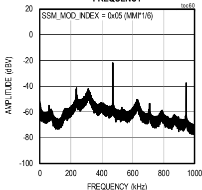
CLASS D OUTPUT FFT vs. FREQUENCY
