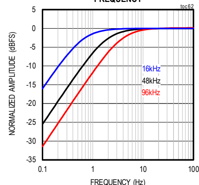
CLASS D DC BLOCKER CORNER FREQUENCY
