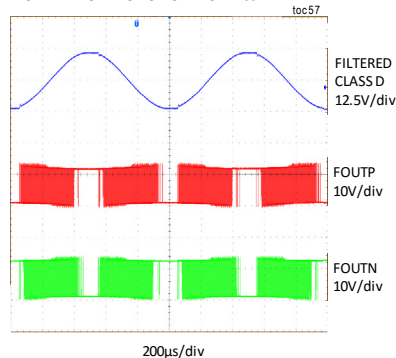
CLIPPING RESPONSE FOR 1% THD+N
