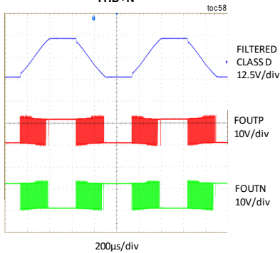
CLIPPING RESPONSE FOR 10% THD+N
