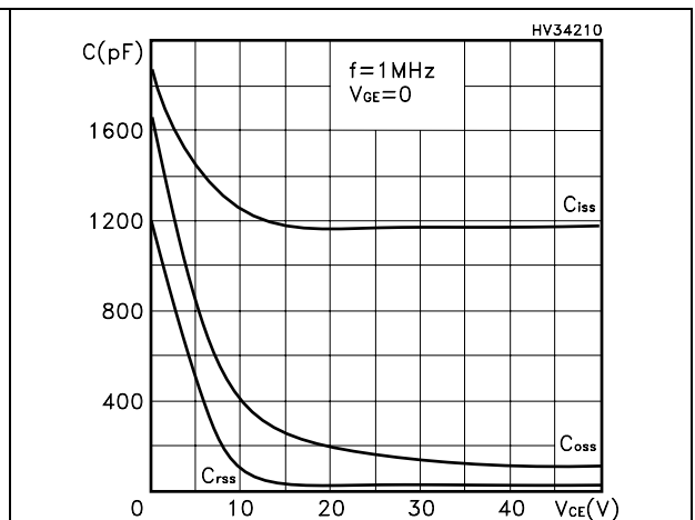
Figure 7. Capacitance variations
